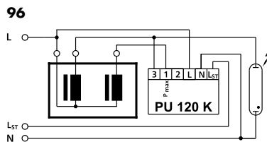
96 Фаза управления отключена (L ST = 0 В) with two ballasts connected in parallel
